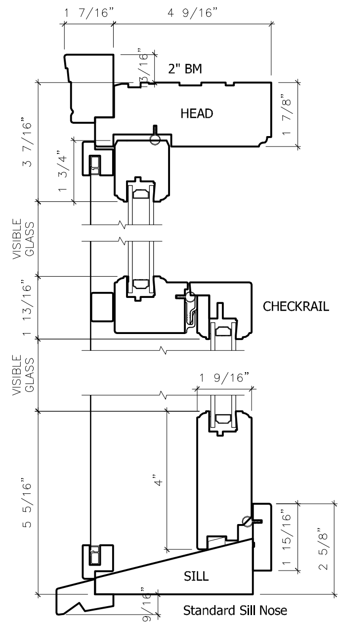
WOOD DOUBLE/SINGLE HUNG LIBERTY - 2" BRICKMOULD 116 (4 3/16") JAMB
