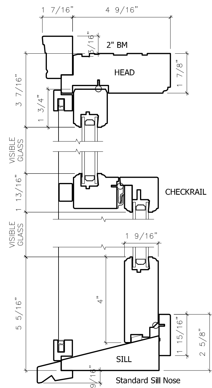
WOOD DOUBLE/SINGLE HUNG - 2" BRICKMOULD 116 (4 3 / 16 ") JAMB
