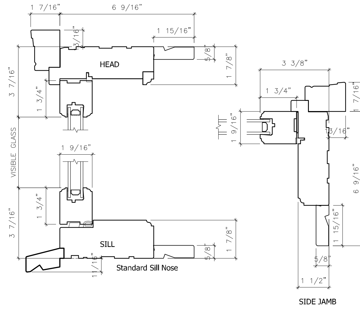
WOOD DOUBLE HUNG TRANSOM 166 (6 9 / 16 ) JAMB
